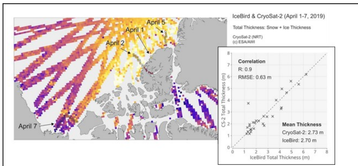
Figure 3.4: Example of collocated sea ice thickness from AWI IceBird airborne EM and CryoSat-2. This comparison show excellent correlation (0.9) using subset of CryoSat-2
