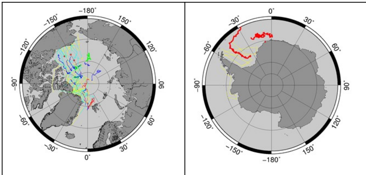
Figure 3.1: Overview of sea ice freeboard, draft and snow depth observations included in the existing RRDP-2; OIB IDCS4 (yellow) and quiklooks (cyan), ULS BGEP (red dots), NP drifting stations (green), IMB CRREL (blue) and Snow depth buoys AWI (red lines).
