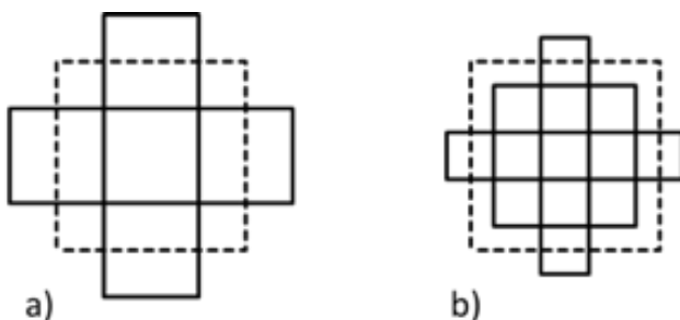
Figure 2.4 Illustration of grid cells used for the 25 km product (a) and the 12.5 km product (b) to approximate the area covered by the 50 km product (dashed square) and compute ~50km averages of the SIC and its retrieval error.
