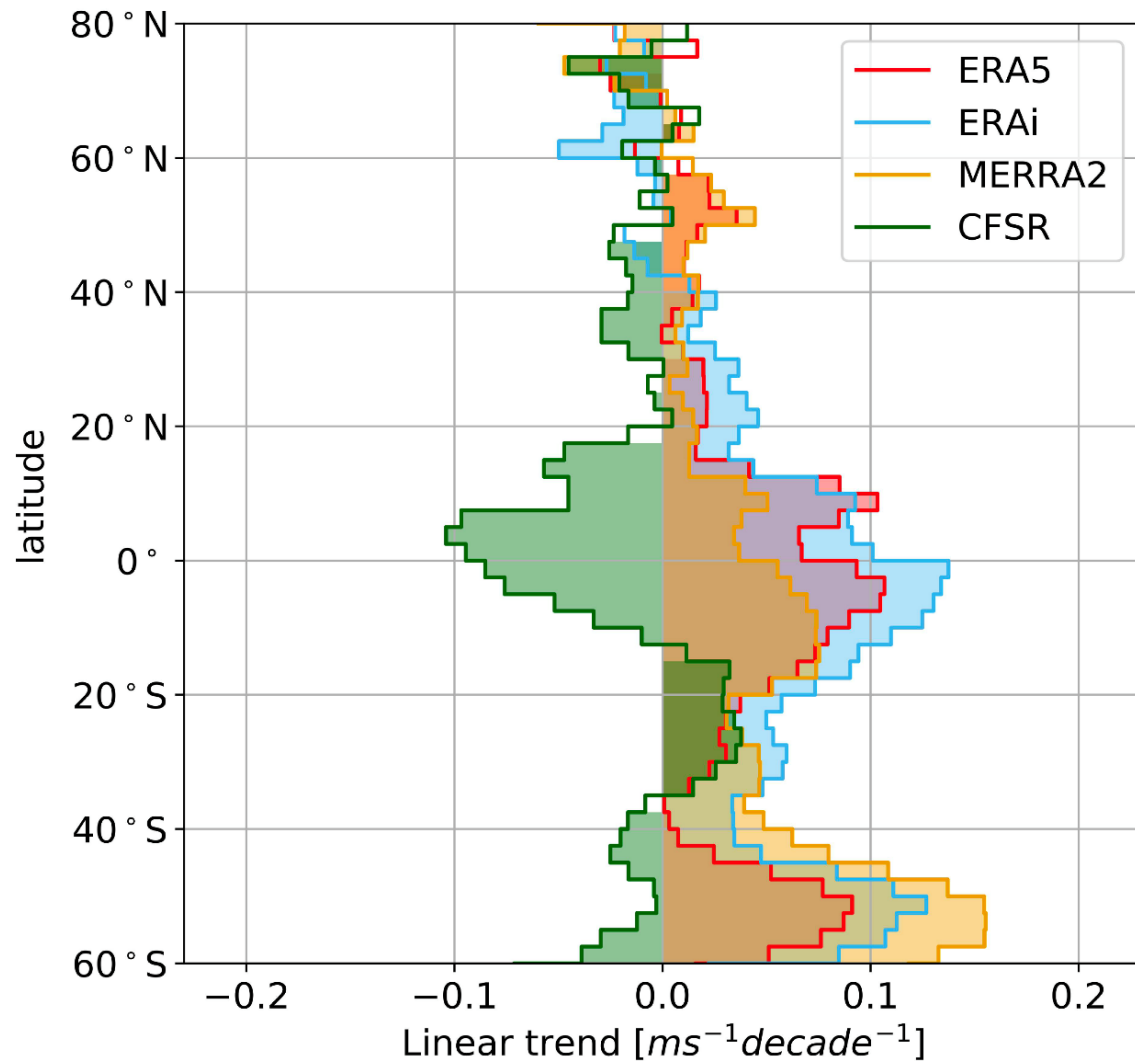
Zonally averaged trends in mean wind speed
