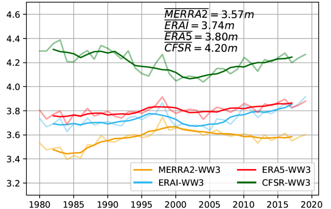
Global 95p SWH for 1980-2019 (5-yr running mean)
