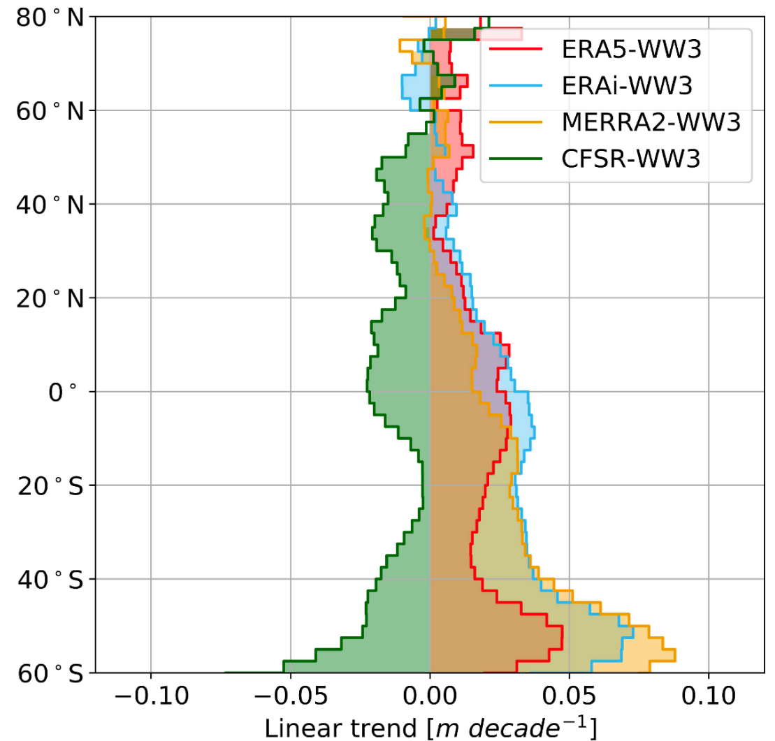
Zonally averaged trends in mean SWH
