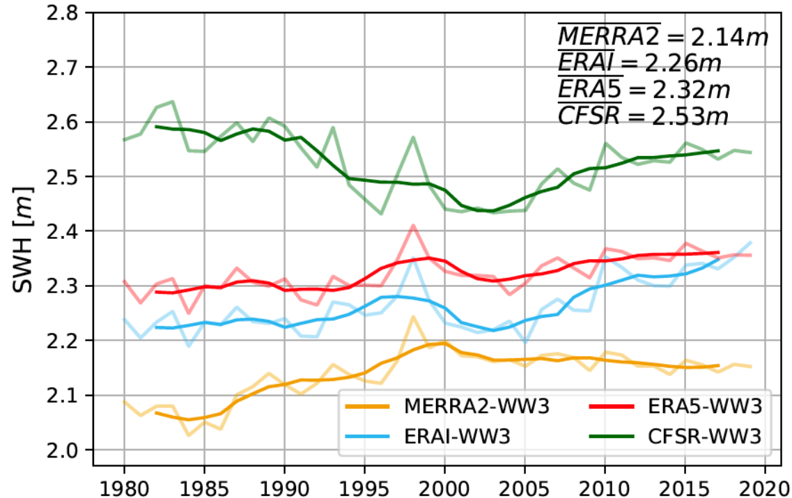
Global mean SWH for 1980-2019 (5-yr running mean)
