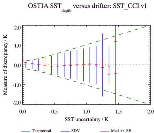
Figure 4-3. Uncertainty validation plot for SST CCI analysis.
