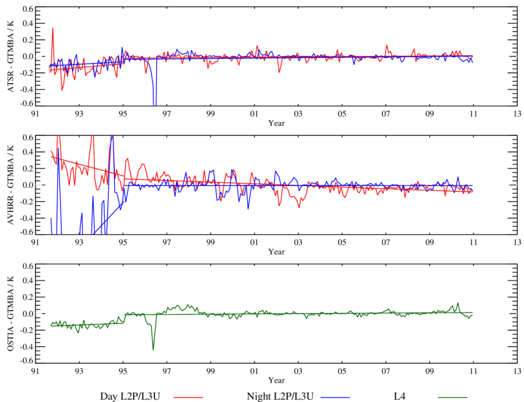
Figure 5-1: Time series of deseasonalised composite monthly mean differences (K) between the SST_CCI products and the GTMBA. Separate day and night time series are provided for the L2P AVHRR and L3U ATSR datasets. Also, plotted are the results of a least squares linear fit for the August 1991 to May 1995 and June 1995 to December 2010 periods (see text for further discussion).
