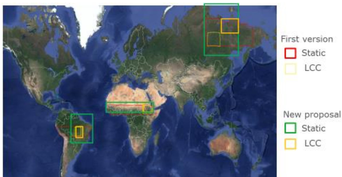
Figure 5: Updated location of the 3 regions as defined in the outcome of the Virtual Meeting to study climate/LC interactions. Newly proposed shapes are superimposed to original ones for better understanding of their differences.
