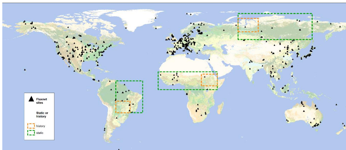
Figure 7. Final selection of the location of the 3 regions to study climate/LC interactions and Fluxnet sites.
