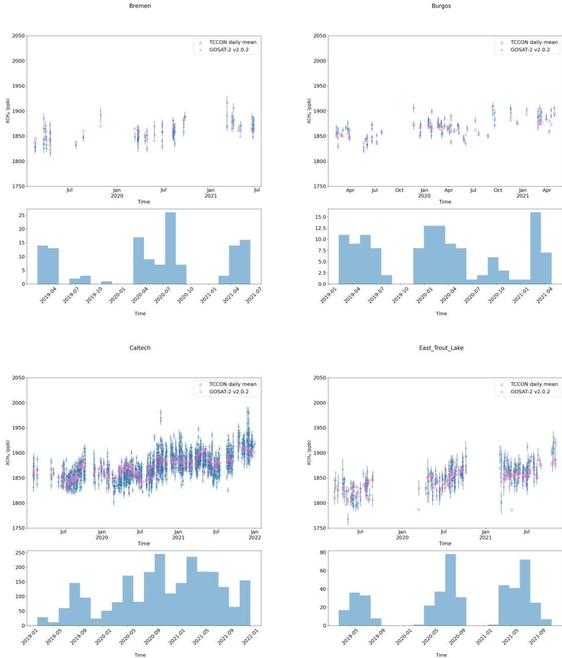
Figure 4.3 Comparison of land single soundings of XCH 4 from the full physics retrieval (blue circles) with co-located TCCON (pink triangles) measurements at all TCCON sites for the period Feb 2019 to Dec 2021. Histograms are also given for each station indicating the number of GOSAT-2 retrievals present throughout the time series.
