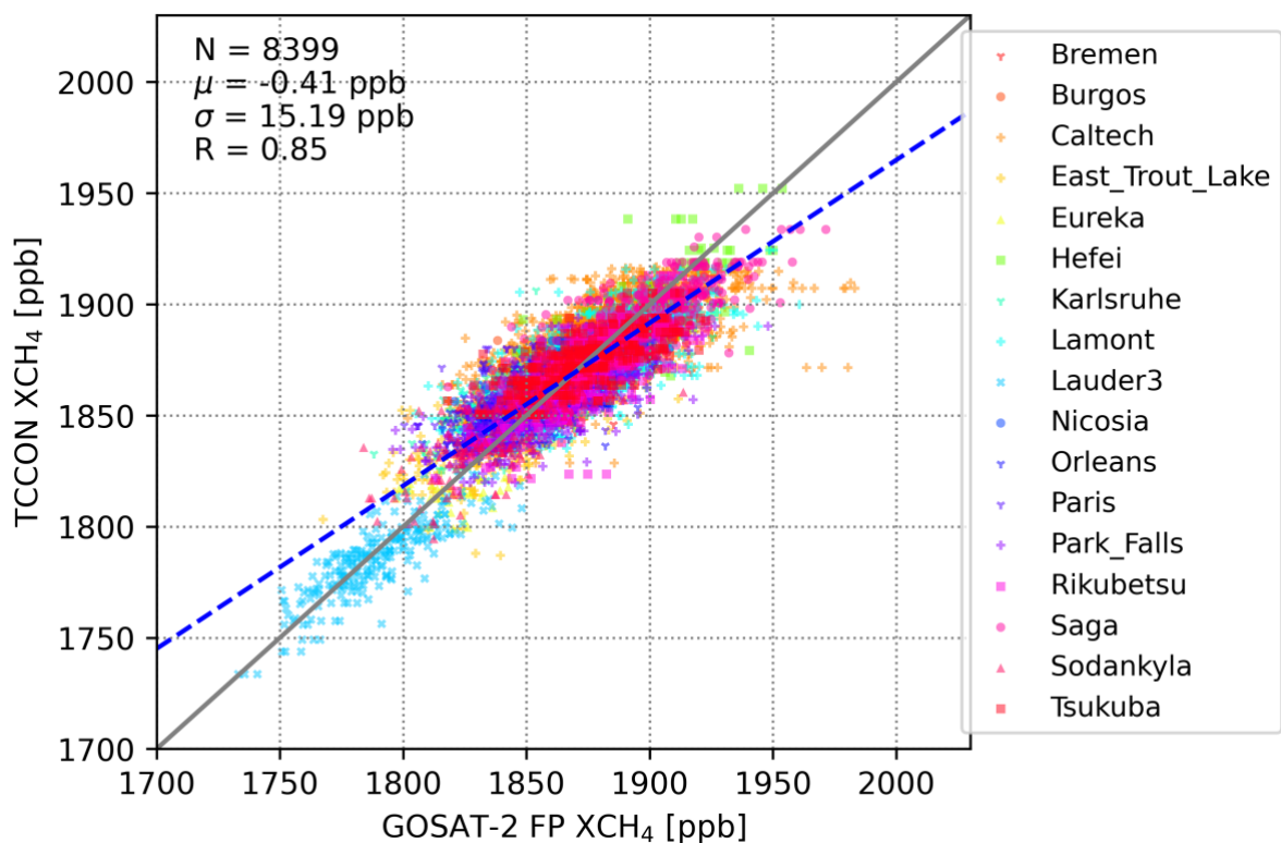
Figure 4.1: Validation of land single soundings of XCH 4 with co-located TCCON measurements at all TCCON sites for the period Feb 2019 to end Dec 2021. Numbers in the figures: \mu = bias, i.e., average of the difference; \sigma = single measurement precision, i.e., standard deviation of the difference; N = number of co-locations; R the correlation coefficient. Stations that are along the coast and also sensitive to glint mode (ocean) measurements are indicated as circles. Those that have high latitudes in the northern and southern hemispheres are upward triangles and crosses, respectively. Stations in Asia, North America and Europe are indicated by squares, pluses and downward triangles respectively. Error bars are not shown due to the large number of data points, however they are of a similar order to those shown in Figure 4.2.
