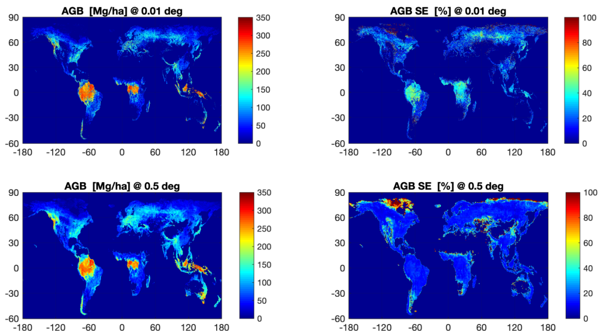
Figure 4-4: Maps of averaged AGB from the CCI Biomass AGB dataset at 0.01° (top left) and 0.5° (bottom left). The corresponding maps of AGB standard error (relative to the AGB value) are displayed in the top right panel (0.01°) and bottom right panel (0.5°).
