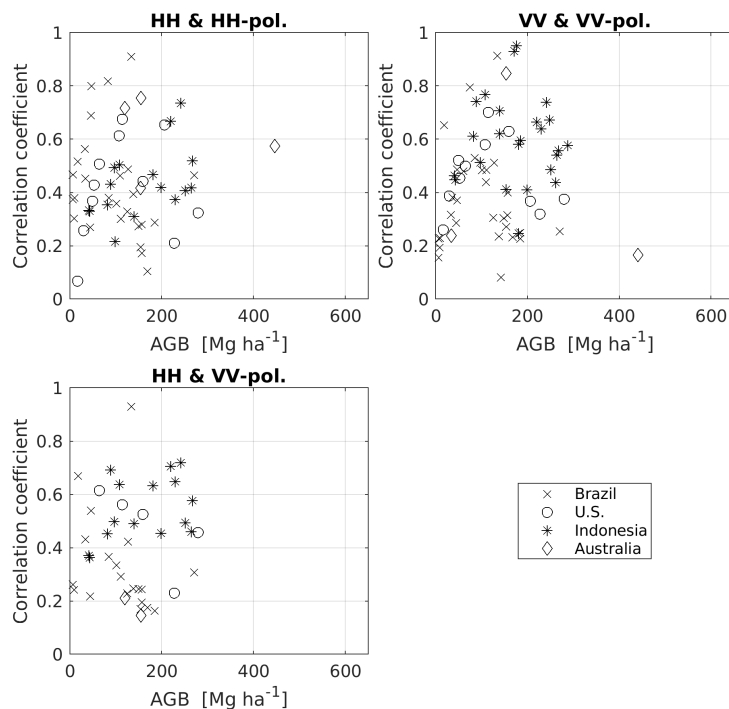
Figure 3-10: Scatterplots comparing the average error correlation per site with the LiDAR-based AGB average. Data points were split depending on the polarization of the first and the second ASAR image.
