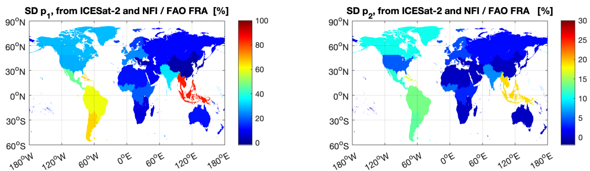
Figure 3-3: Maps of the standard deviation of coefficients p_1 and p_2 . The maps show the ratio between the standard deviation and the estimate of each coefficient. Maps of the two coefficients are displayed in [RD-3].
