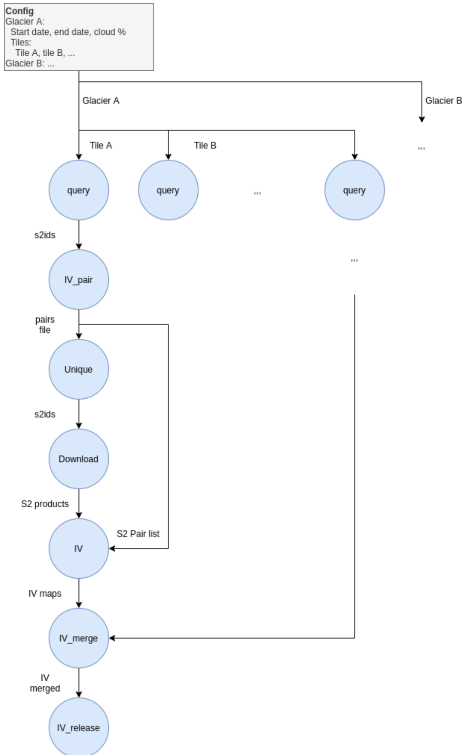
Figure 4.1: Optical IV processing pipeline. Multiple glaciers can be configured, and for each glacier a subgraph of tiles is generated over which optical IV is measured and finally merged into the final IV release product.
