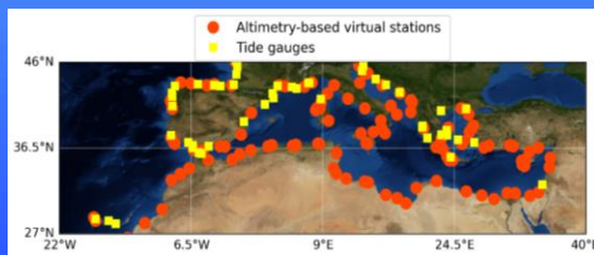
Virtual stations in the Mediterranean Sea (red dots) with tide gauge sites superimposed (yellow squares)
