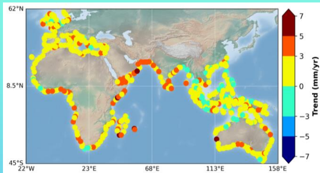
The 620 altimetry-based virtual coastal stations. Colors represent coastal sea level trends (mm/yr) over 2002-2020
