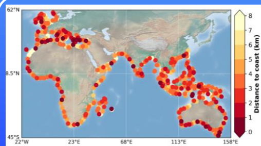
Closest distance (km) to the coast of the first valid point along the Jason track for all 620 virtual stations
